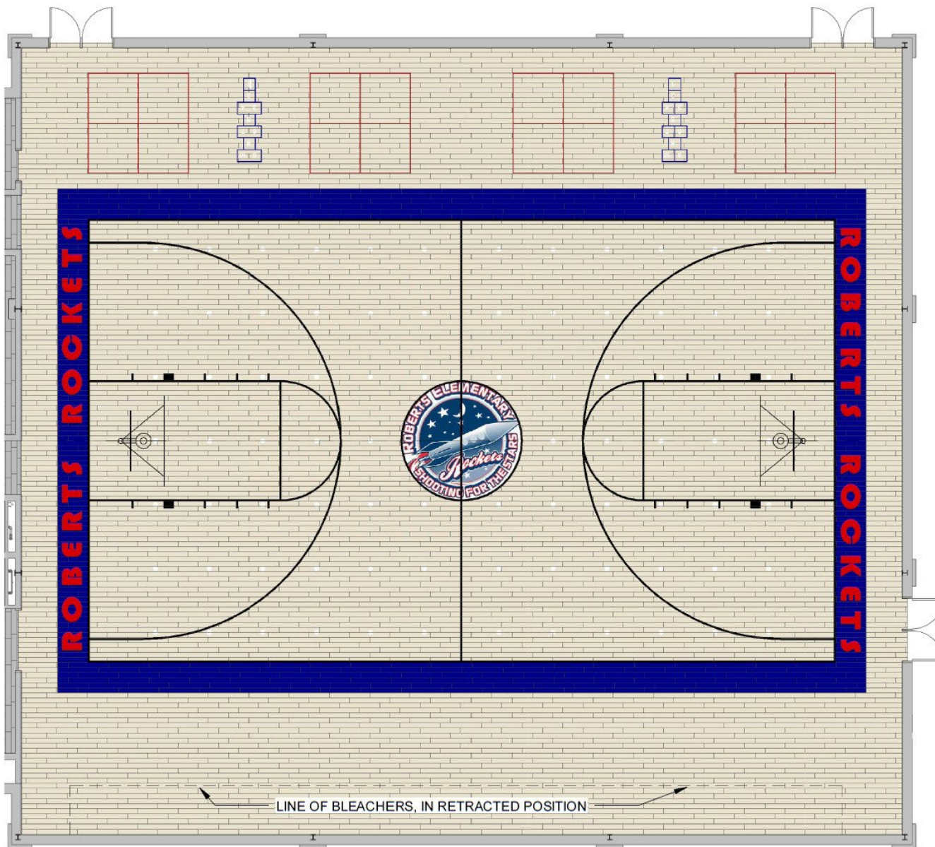
GYMNASIUM FLOOR PATTERN PLAN
